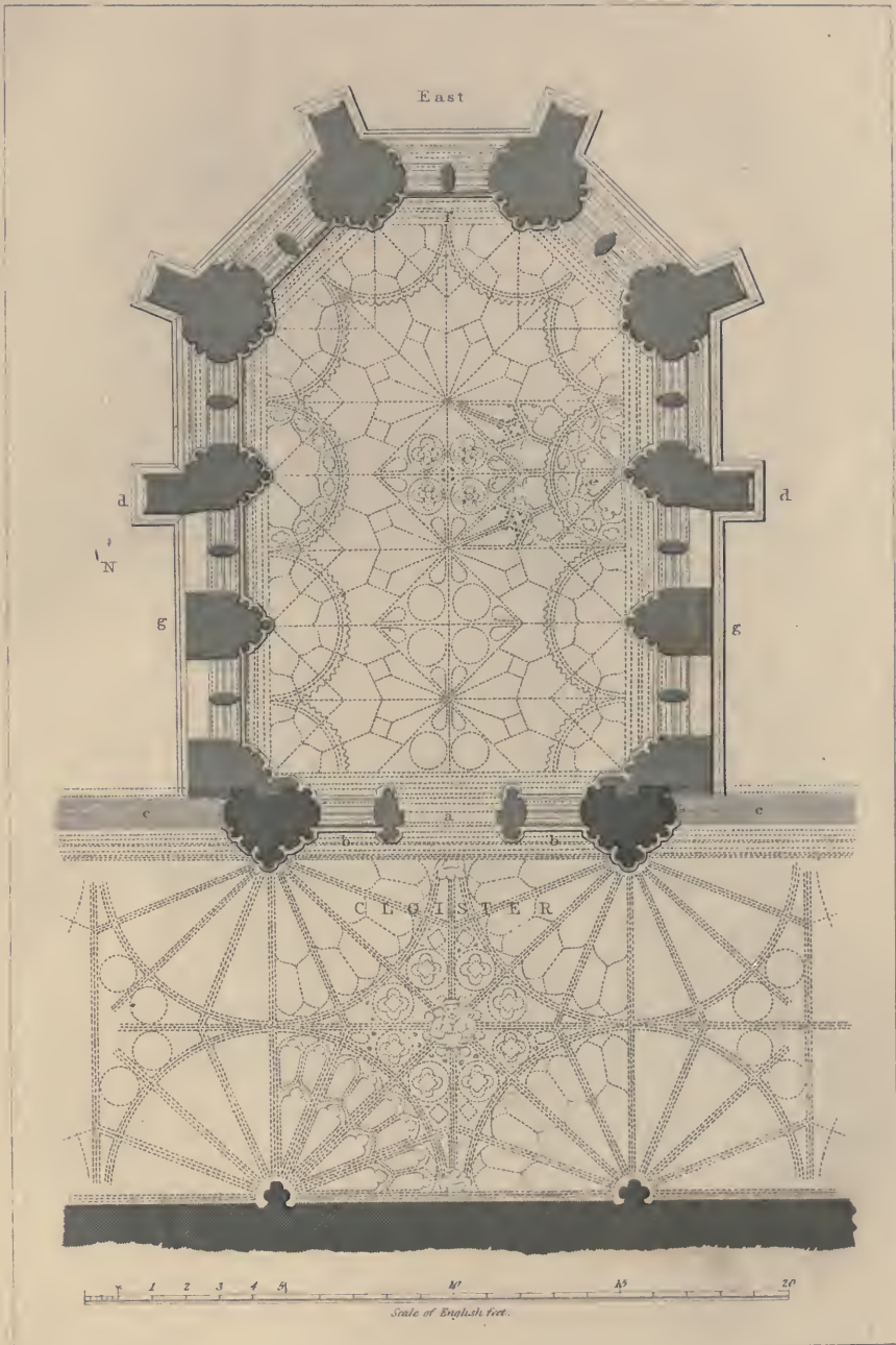
GROUND PLAN CHANTRY-CHAPEL &c ST STEPHEN'S CHAPEL WESTMINSTER.
